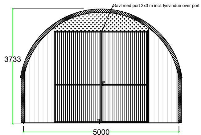
Facade port gavl 3x3 m:
